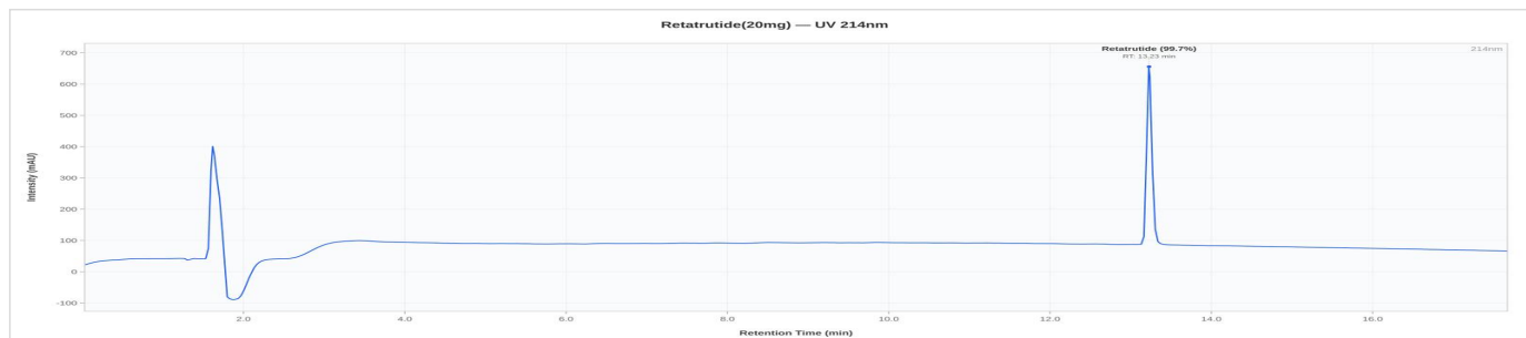
GLP-3(R) 20mg - RT20-1007: UV Chromatogram
